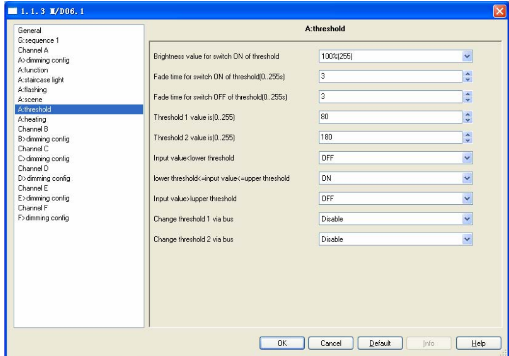
Fig4.4: “threshold” window
