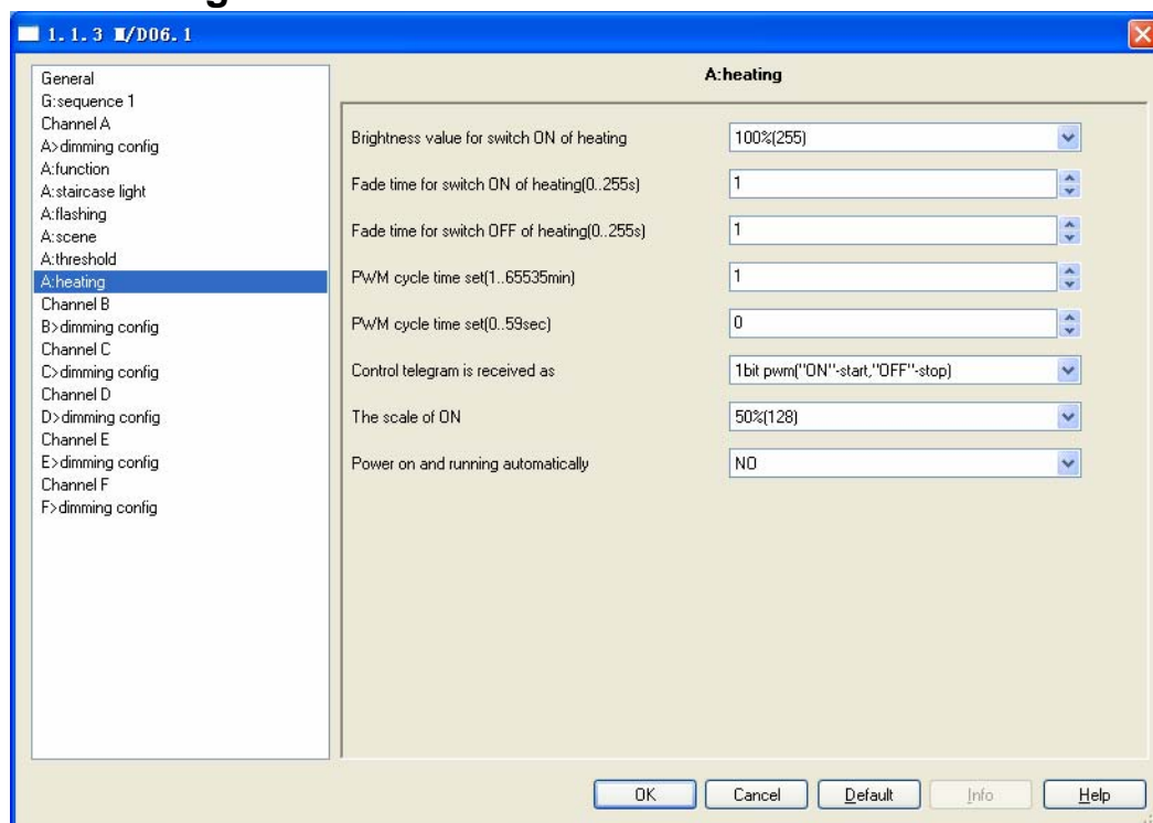
Fig4.5: “heating” window
