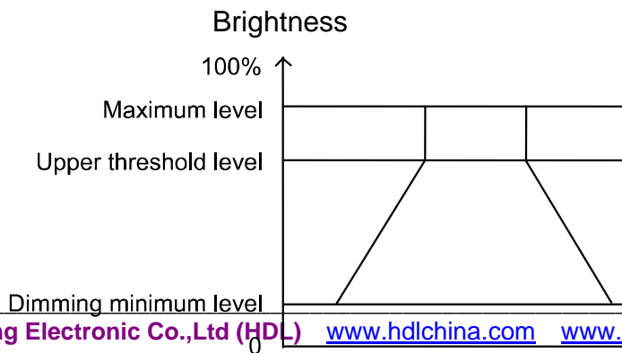
Fig 2.5 Switch ON/OFF or Absolute dimming
